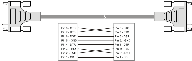
Figure 12. 4310-0061 cable
